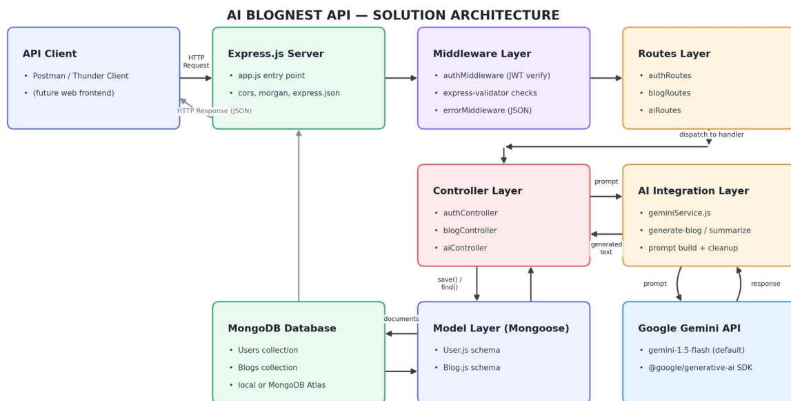
Figure 1: Architecture and data flow of AI BlogNest API
